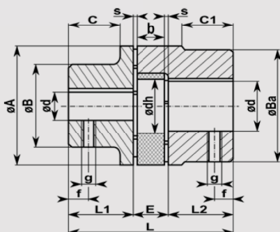
Hub combination A/B e.g. Coupling 28/38 – 28/35
