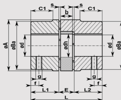
Hub combination B/B e.g. Coupling 28/38 – 38/38
