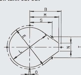
Oil tank cut-out
