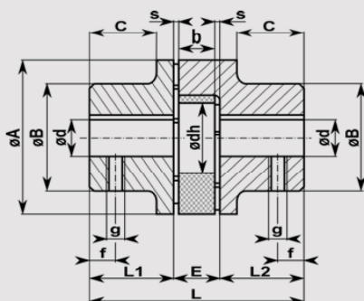
Hub combination A/A e.g. Coupling 28 – 28/20
