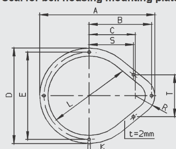
Seal for bell housing mounting plate
