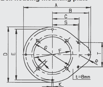
Bell housing mounting plate
